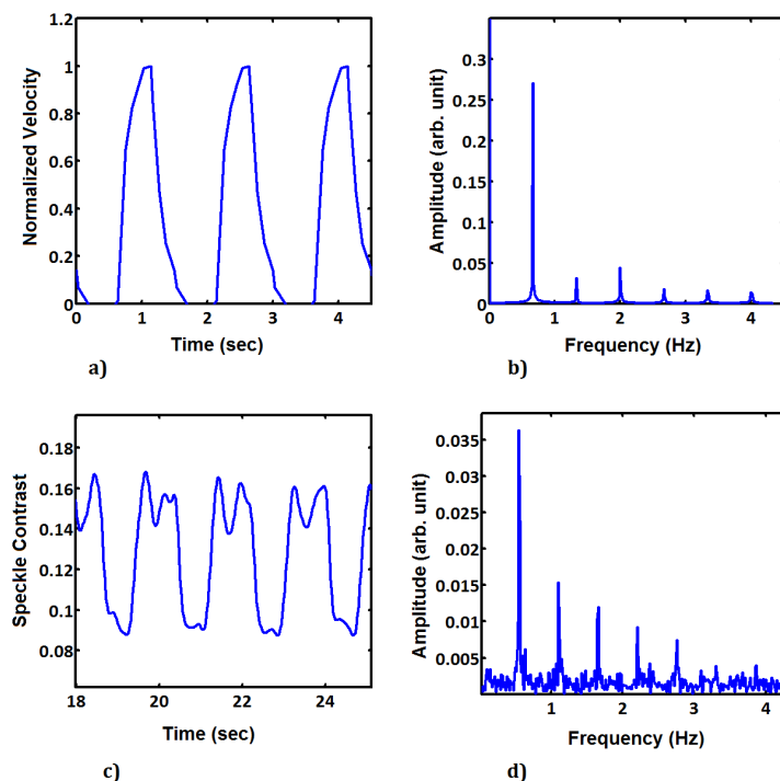
Fig. 5 Time sequence of PIV (a) and LASCA (c) generated from images recorded during pulsatile flow in the cylindrical phantom. Frequency spectrum extracted from the time sequence for PIV (b) and LASCA (d) measurements
