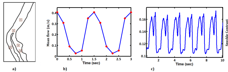
Fig. 6 a) The selected zones for analysis from Carotid Artery Phantom. b) Time sequence for PIV , c) Time sequence for LASCA, in zone 2.
