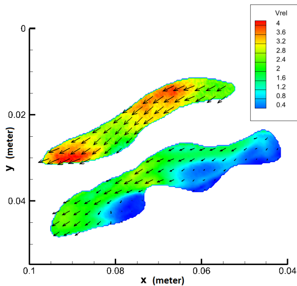
Fig. 4 Final velocity map of the carotid artery phantom. Color indicates the velocity vectors amplitude. V_{rel} is the dimensionless velocity defined as ratio of velocity and mean inflow velocity.
