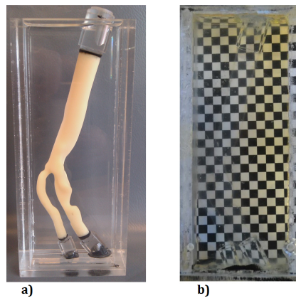
Fig. 2 Flow phantom of patient based carotid artery: a) in water and b) with index matched solution
