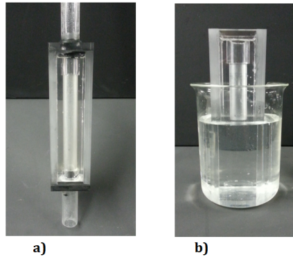
Fig. 1 Straight cylindrical flow phantom: a) in water and b) with index matched solution
