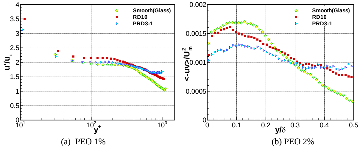
Fig. 3 Comparison of turbulent quantities in low-Reynolds number flow for FDR-SPC
