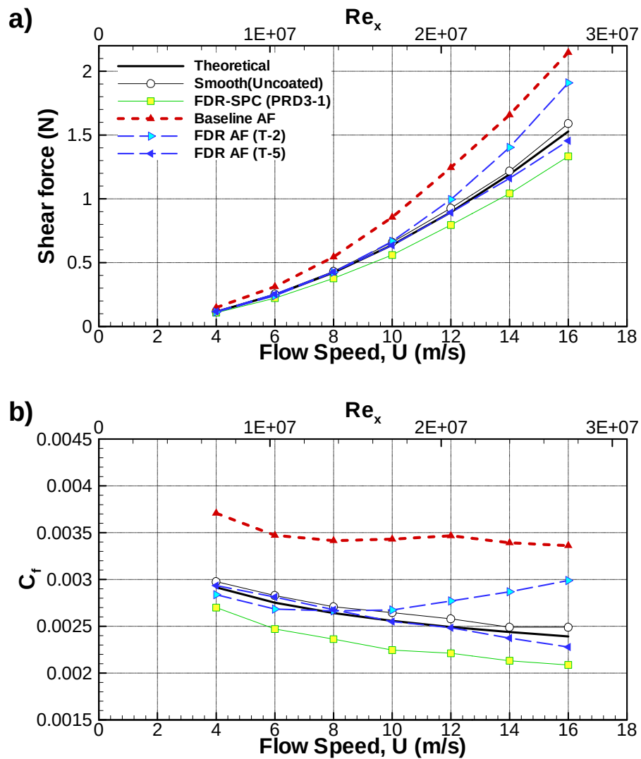
Fig. 5 Comparison of frictional drag in high Reynolds number flow for FDR-SPC and FDR AF coatings
