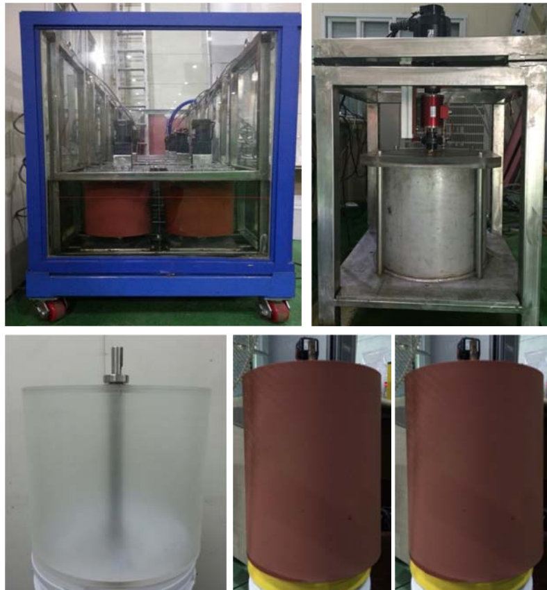
Fig. 7 Photos of rotor test apparatus and rotors with different coatings
