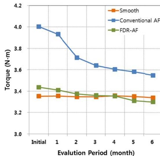
Fig. 8 Long-term temporal variation of torques of rotors with varying surface conditions
